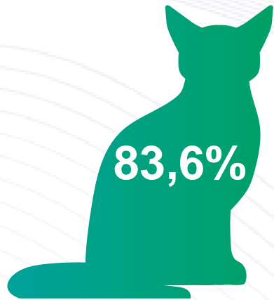
of cat (hair) allergen Fel d1
